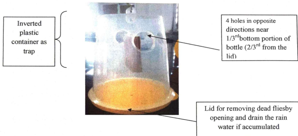
Fig-3 Trap assembly with killing block
